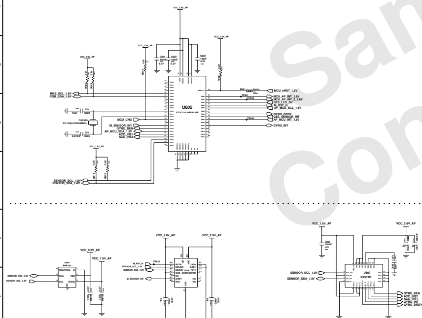
Barometer Sensor
