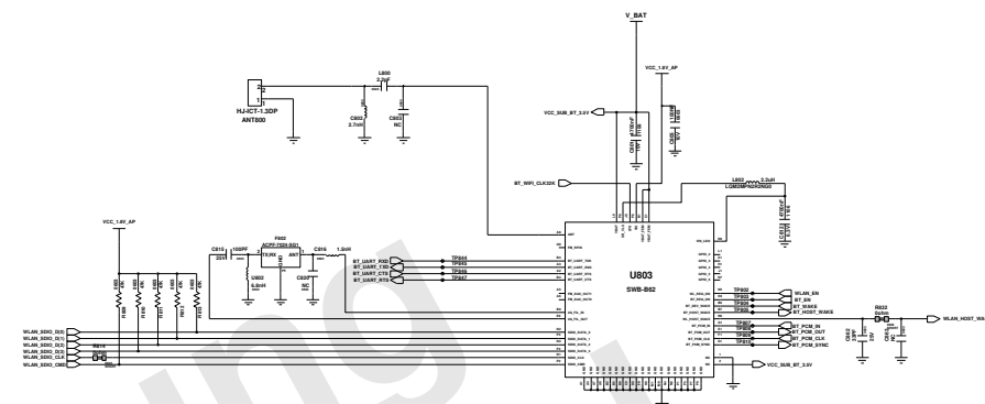
BT / WIFI
